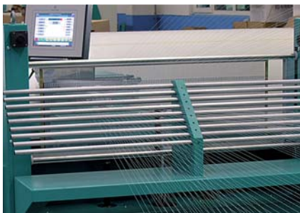
Leasing device Gelesevorrichtung
