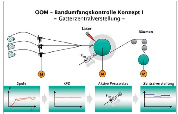
Regulation system 2 Regelsystem 2
